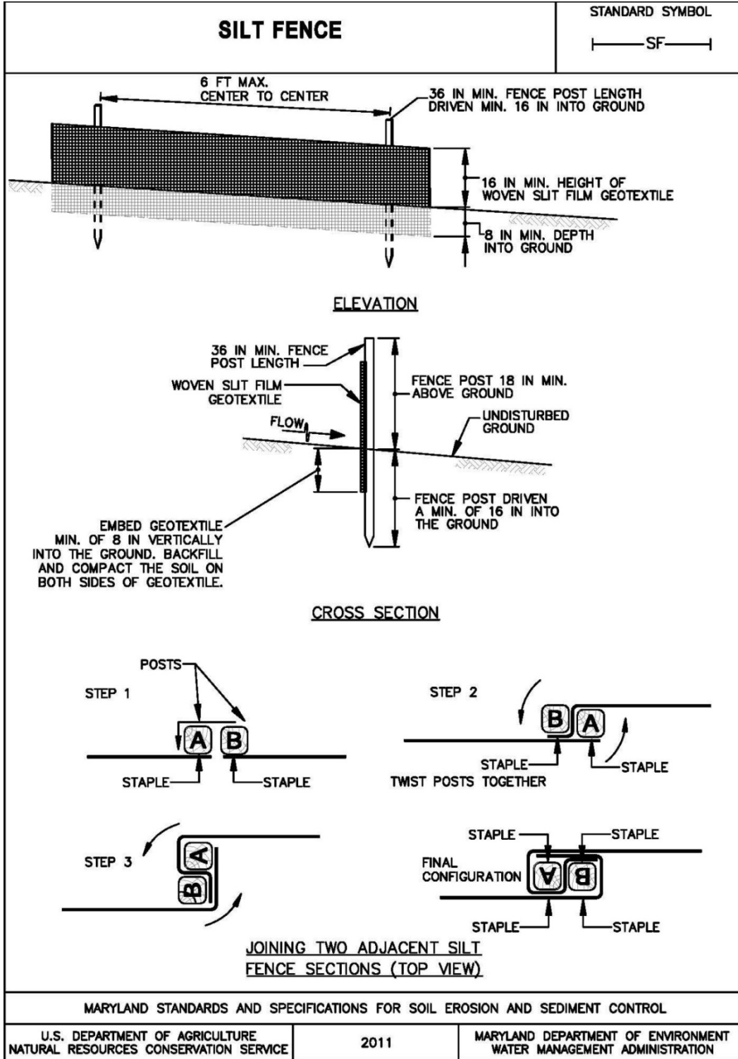
Diagram 15.0 Silt Fence
