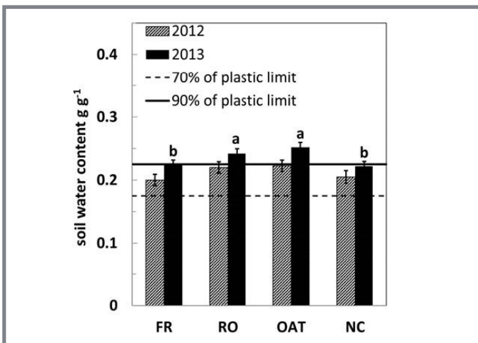
Figure 2: Soil gravimetric water content (0-8") in early April at Wye Research and Education Center, a moderately well drained silt loam. The 70-90% plastic limit is the water content at which the least amount of structural damage occurs from traffic and/or tillage. FR= forage radish, RO= radish/oat mix, OAT= oat, NC= no cover crop (tilled in November). Oat, a high-residue cover crop, increased the soil water content to the point at which traffic and tillage would likely cause damage. (Lounsbury and Weil, 2015).
