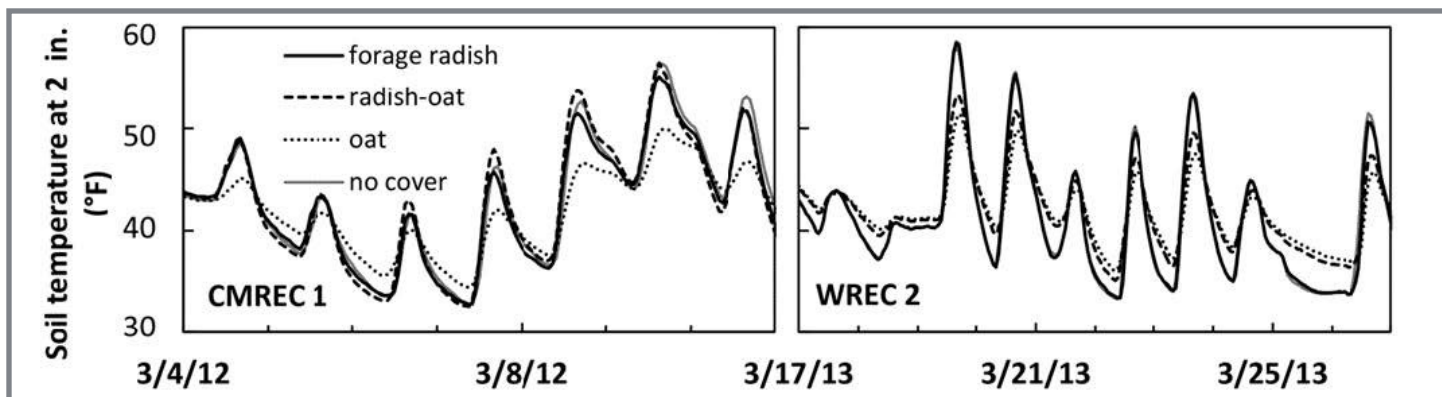
Figure 4: Soil temperature fluctuations for untilled soil in March at Central Maryland Research and Education Center, Clarksville (CMREC), and Wye Research and Education Center (WREC). Residue from oat moderates the daily high and low temperatures. The daily high temperature after radish is comparable to having no cover crop.
