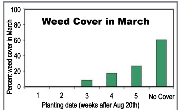
Figure 1: There was complete weed suppression in March when a forage radish cover crop was seeded one and two weeks after August 20. Spring weed cover increased following later forage radish plantings. Although weed suppression is greater after a forage radish cover crop seeded five weeks after August 20 than after no cover crop, the weed suppression is not adequate for no-till spring seeding without herbicides. (Lawley and Weil, unpublished).
